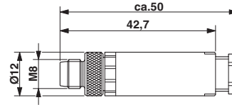
M8 x 1 male connector, straight version
