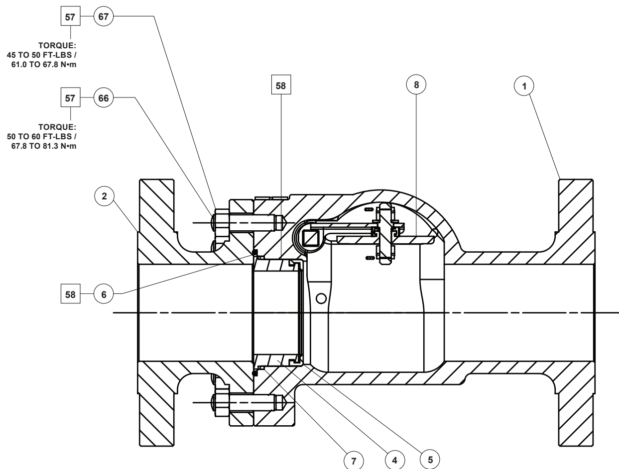
Figure 9. Types N551-24F and N551-16F Flange Body Mounted with Flange with Mounting Studs and Nuts
