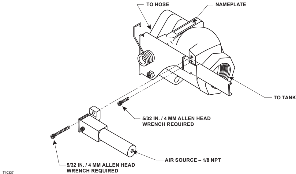
Figure 6. Type P327D Pneumatic Cylinder Installation
